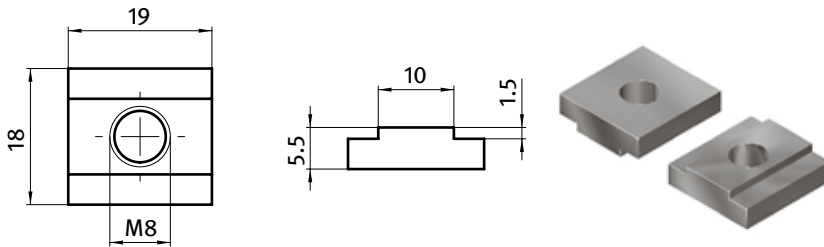
Nutenstein T-slot Nut
